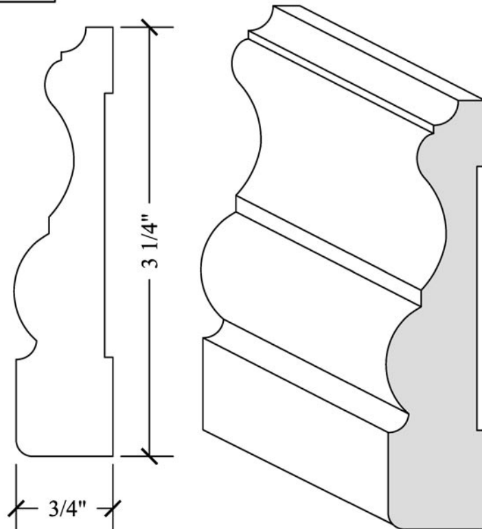
CASING 3/4" x 3-1/4"
