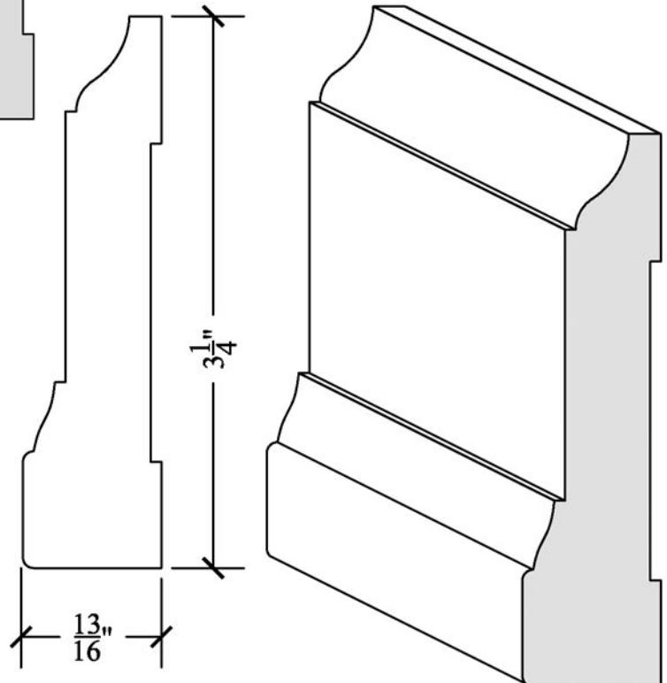
CASING 13/16" x 3-1/4"
