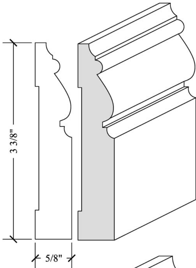
BASE 5/8" x 3-3/8"
